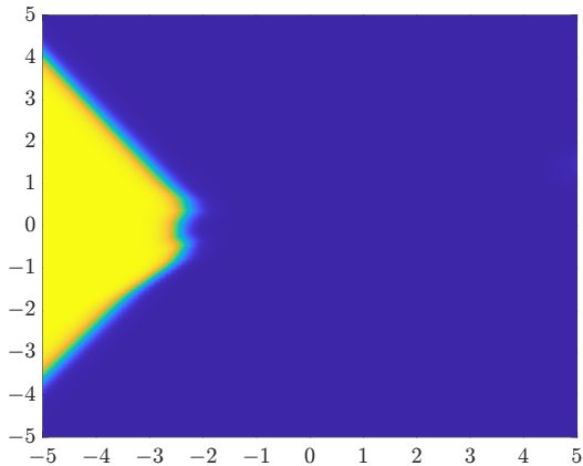
Figure 4. Double-dual density \hat{\phi}_j^* over X associated to x_j = (0, 0) with class y_j = 1 .
